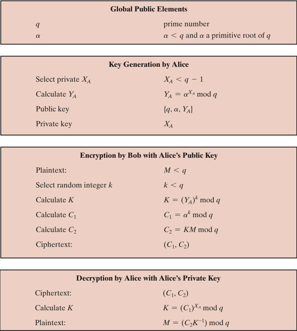
Figure 10.3 The ElGamal Cryptosystem
