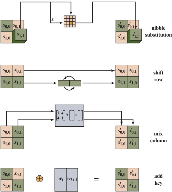
Figure D.4 S-AES Transformations
