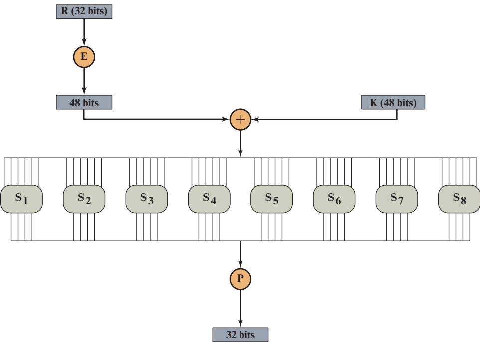
Figure C.3 Calculation of F(R, K)
