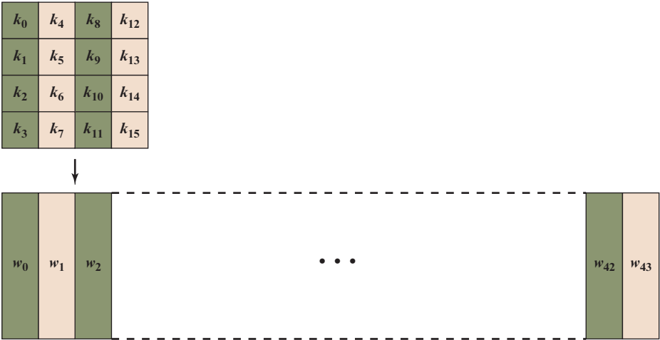
(b) Key and expanded key
