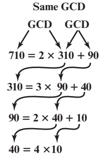
Figure 2.3 Euclidean Algorithm Example: \gcd(710, 310)
