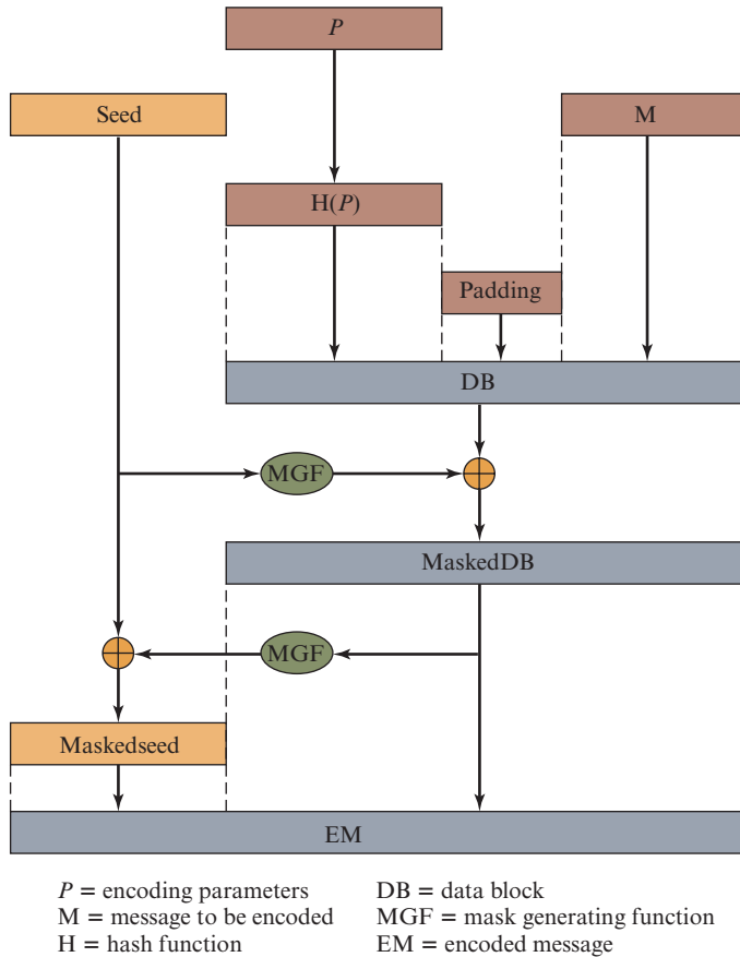
Figure 9.9 Encryption Using Optimal Asymmetric Encryption Padding (OAEP)
