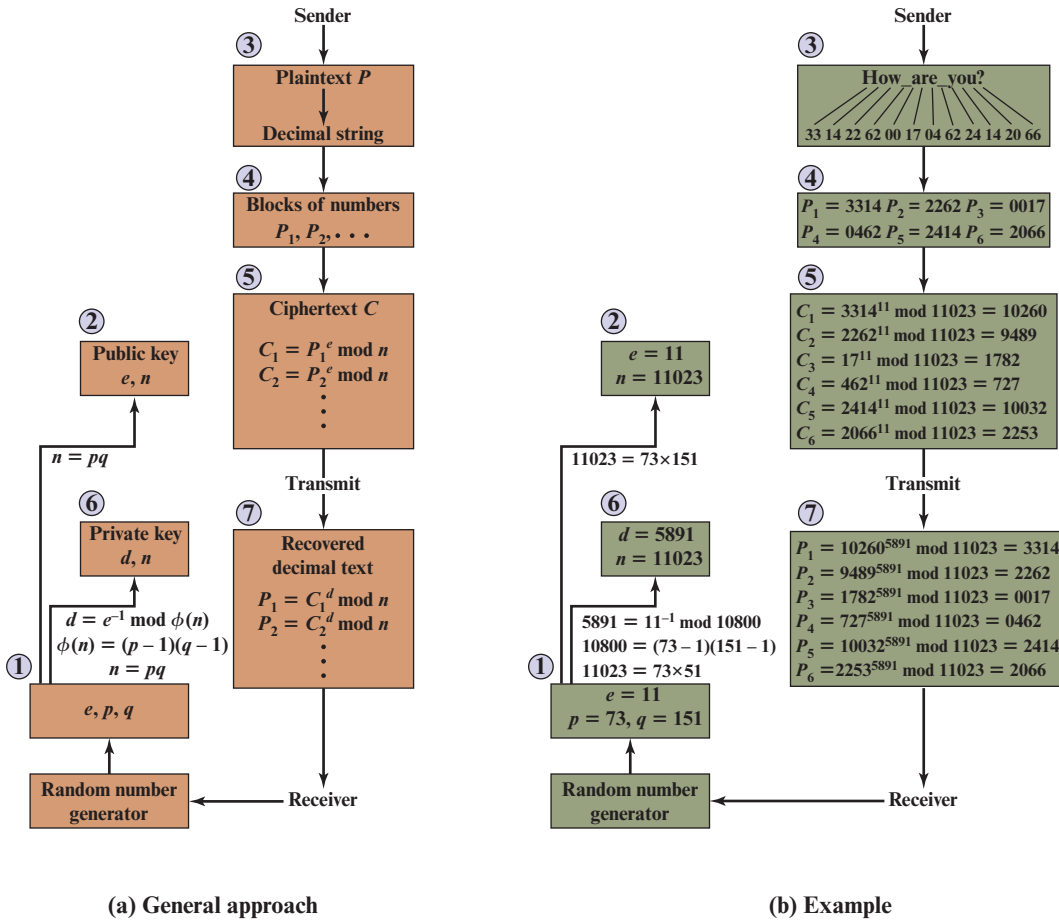
Figure 9.7 RSA Processing of Multiple Blocks
